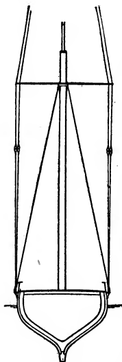
TOPMAST RIGGING.
